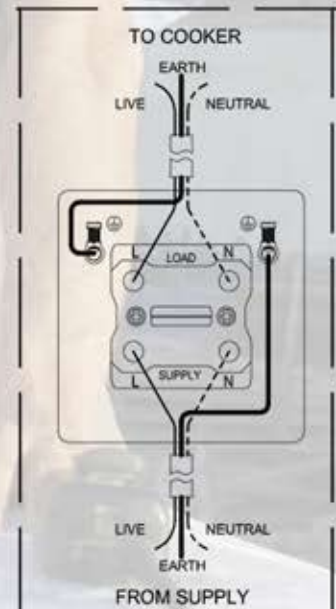
45A SWITCH
