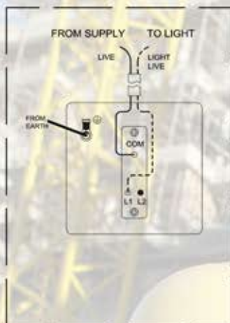
1 WAY SWITCH
