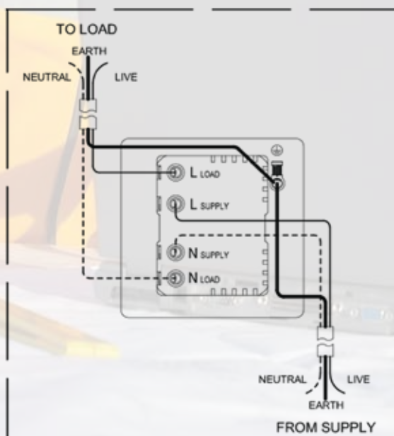
32A KEYKARD SWITCH
