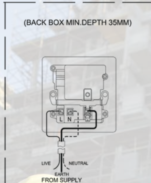
13A 1 GANG SOCKET WITH USB OUTLET
