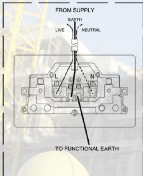
2 GANG MULTI FUNCTION SOCKET
