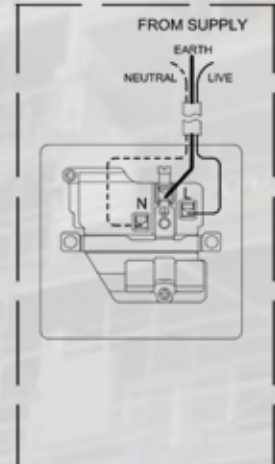
13A 1 GANG SWITCHED SOCKET
