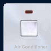
MT5217: 45A, double pole switch, marked "Air Conditioner" with neon, 1 gang
